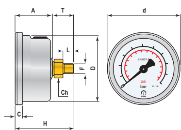
P-Type stem mounted, centre back connection
