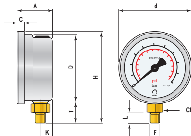
R-Type stem mounted, bottom connection
