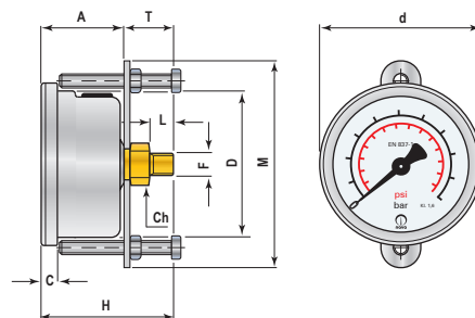
S-Type panel mounted with clamp, centre back connection
